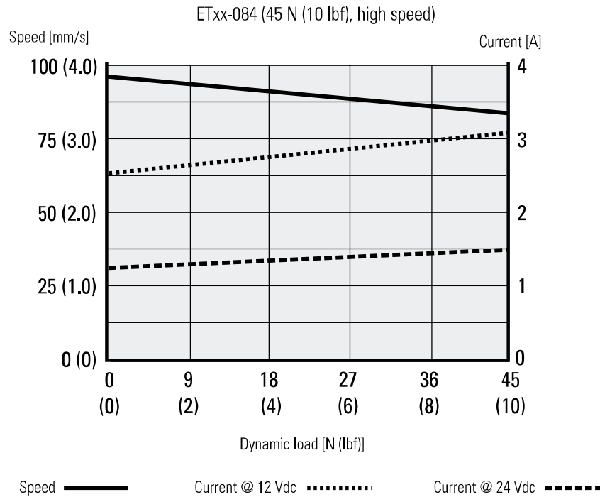
Speed and Current vs. Load
